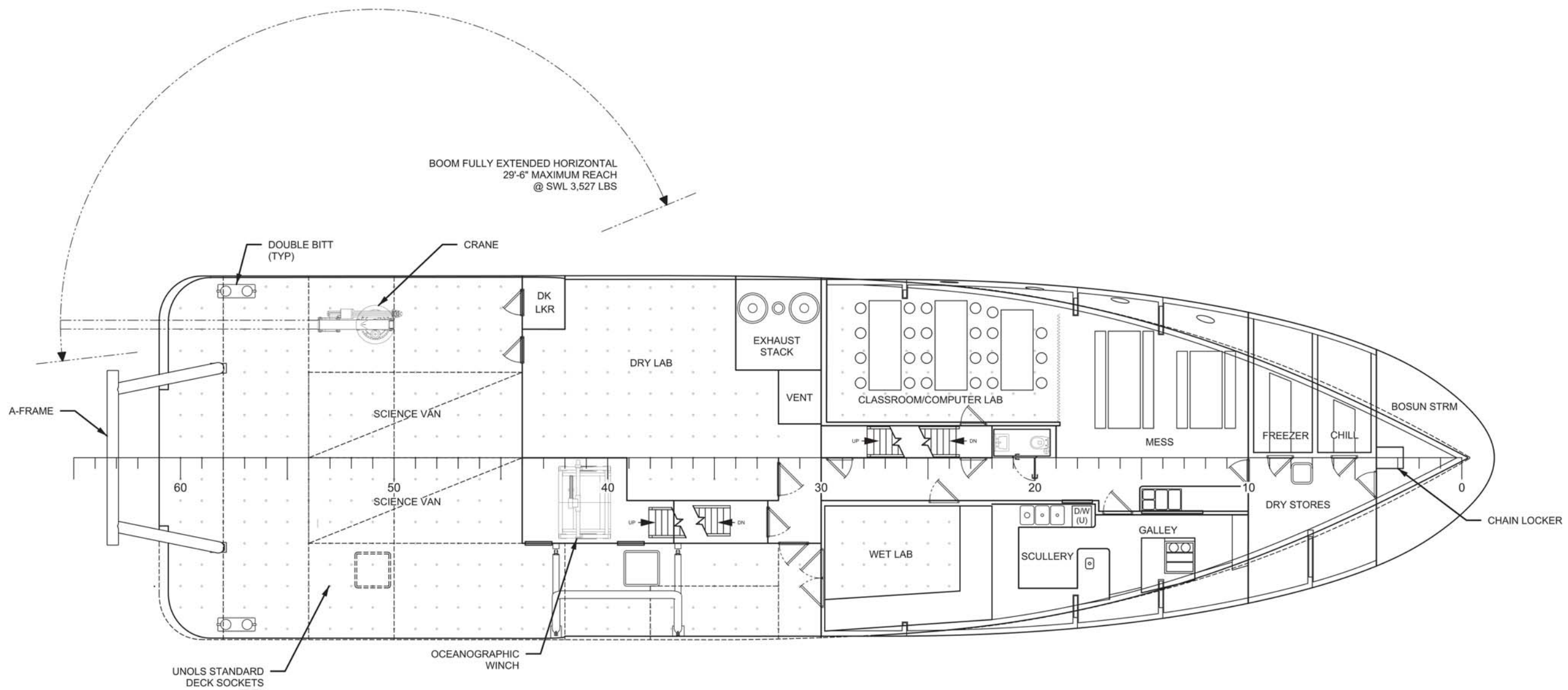
PLAN 3-5B MAIN DECK 3/32"=1'-0"
