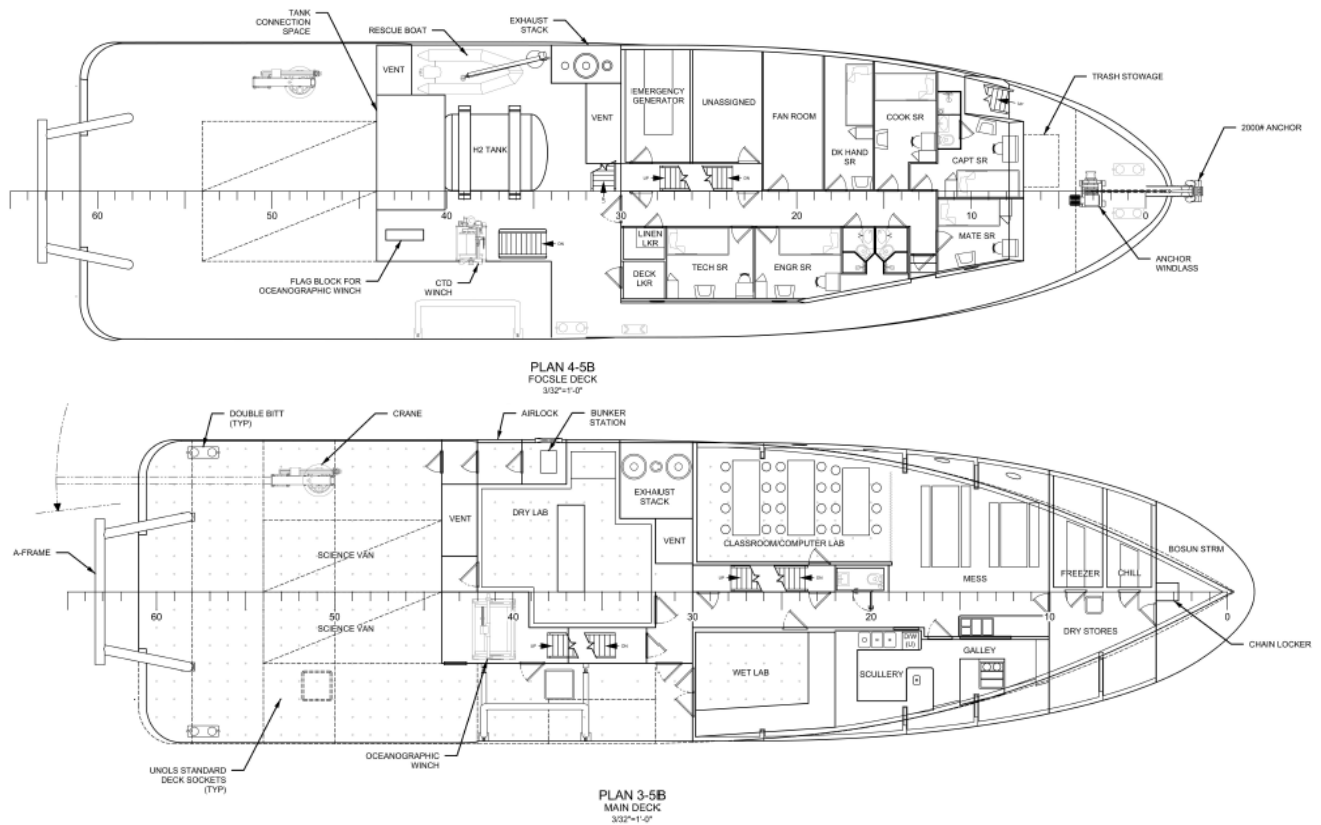
Figure 15 Hydrogen hybrid SRV Main and Focsls Decks
