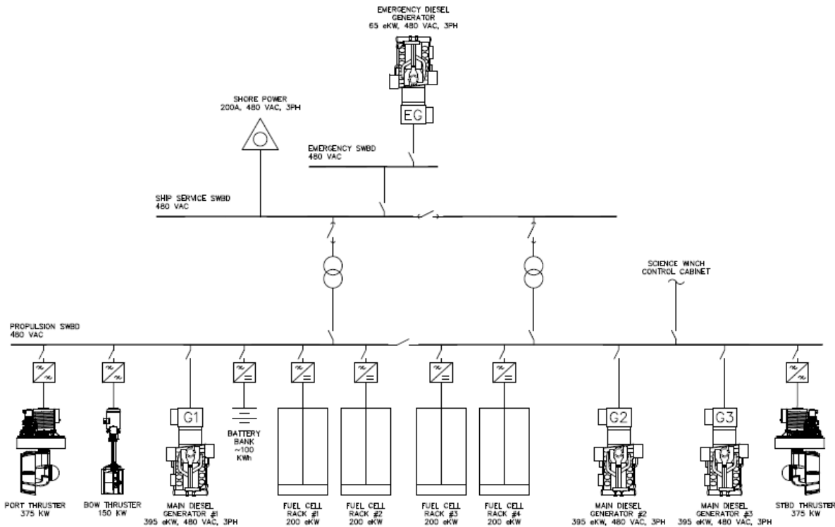
Figure 17 Propulsion system block diagram
