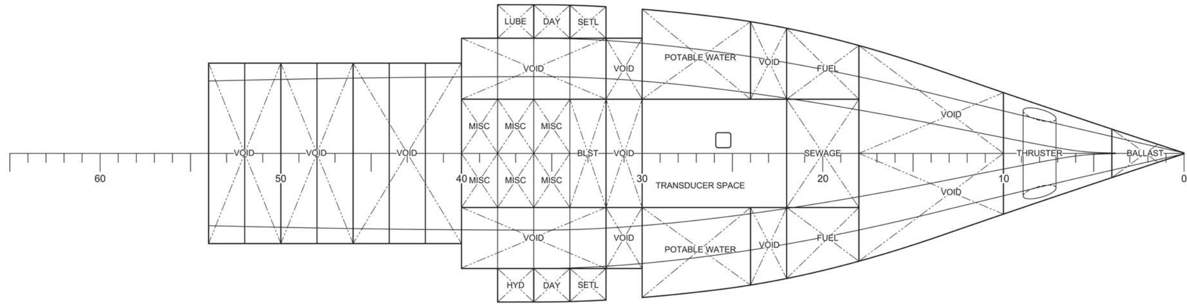
PLAN 2-5C TANK PLAN 3/32"=1'-0"
