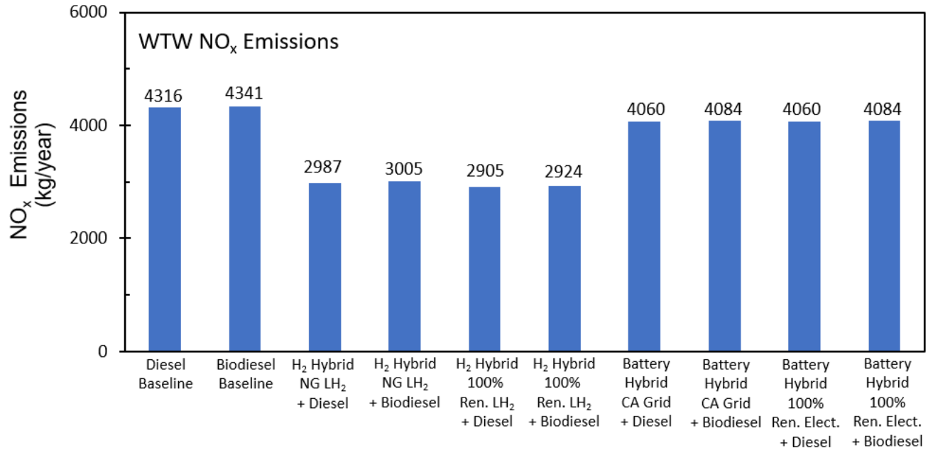
Figure 4: Predicted annual well-to-waves (WTW) NO x emissions for the Diesel Baseline vessel, Biodiesel Baseline vessel and the Hydrogen (H 2 ) Hybrid vessel, with NG LH 2 and 100% renewable LH 2 accompanied by diesel power from fossil diesel and biodiesel. Also shown are the predicted annual NO x emissions for the Battery Hybrid with CA Grid and 100% Renewable shore power accompanied by diesel and biodiesel fuel for the diesel generator portion of the hybrid propulsion system. The diesel and biodiesel engine emissions are constrained to the Tier 3 limits.
