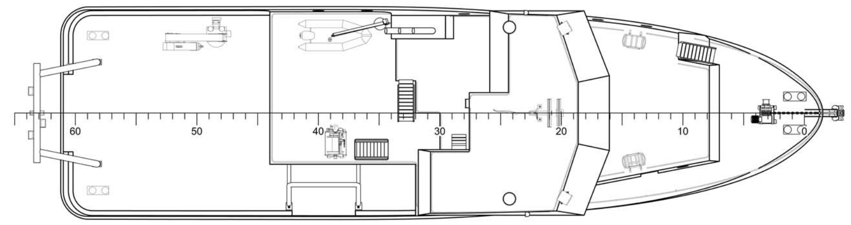
PLAN 1-6A WEATHER DECKS 1/16"=1'-0"
