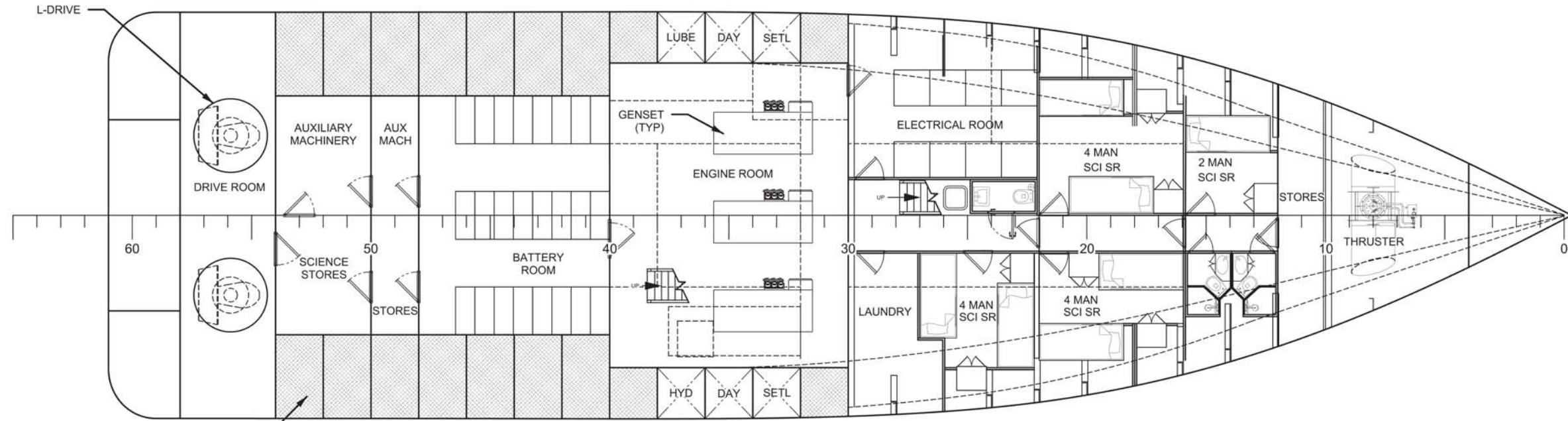
PLAN 2-5A 1ST PLATFORM 3/32"=1'-0"
