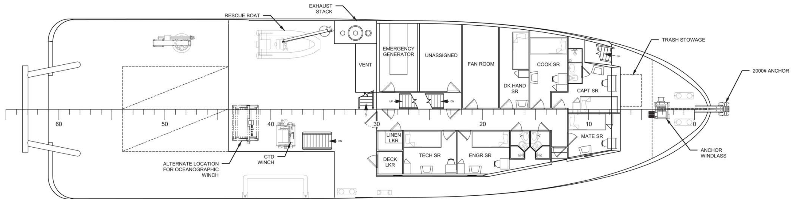
PLAN 4-5B FOCSLE DECK 3/32"=1'-0"
