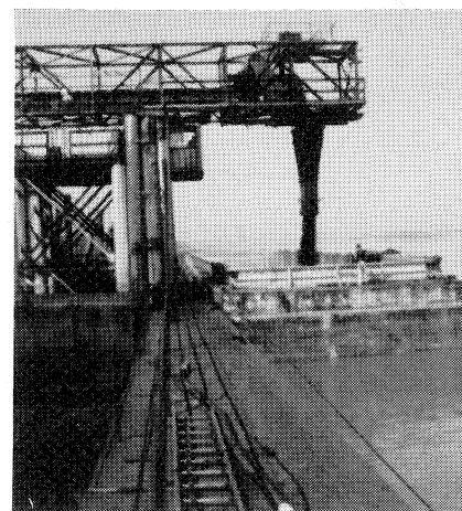
Coal moves from railroad car (not shown) on conveyor belt (top) into barge at American Terminal operated by American Commercial Barge Line Co. on the Ohio River at Louisville, Ky. Coal transfer system is one of four operated by company on Ohio and Mississippi Rivers.
